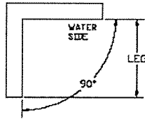
90° Single Weld
