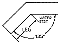
135° Single Weld
