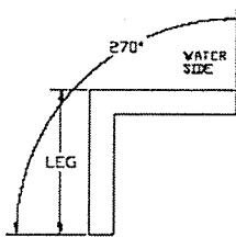
270° Single Weld
